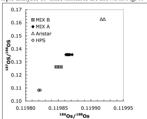
Figure 1: External reproducibility of 186 Os/ 188 Os and 187 Os/ 188 Os analyses by MC-ICP-MS on synthetic reagent mixtures from Oct. 2007 to Dec. 2007.
