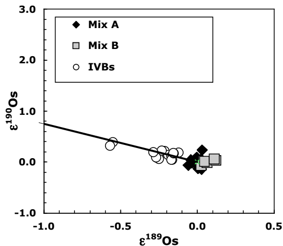
Figure 2: Replicate 189 Os/ 188 Os and 190 Os/ 188 Os of 6 group IVB irons, and two terrestrial standards (Mix A, Mix B). The line represents cosmic-ray neutron capture burn-out of Os.
