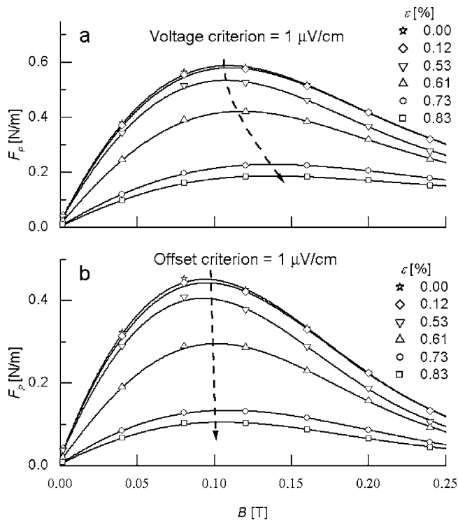
FIG. 4. (a) Macroscopic pinning force of tape B-3 as function of magnetic field for different applied strains when the critical current is determined with a voltage criterion of 1 \mu\text{V}/\text{cm} . The arrow indicates the shift of the maximum pinning force to higher magnetic field as the strain exceeds \varepsilon_{\text{irr}} = 0.53\% . (b) F_p , when the critical current is determined with an offset criterion at 1 \mu\text{V}/\text{cm} , shows the absence of any shift when current sharing is corrected.
