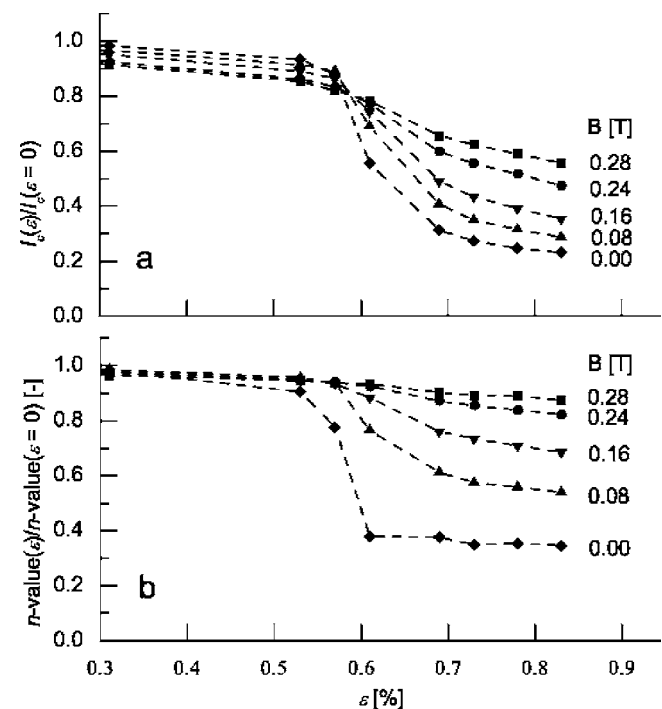
FIG. 3. (a) Normalized critical current of tape B-3 as function of tensile strain at 77 K for different magnetic fields applied perpendicular to the wide side of the tape, showing a greater strain effect at low magnetic fields. (b) Normalized n value as a function of the tensile strain and magnetic field.
