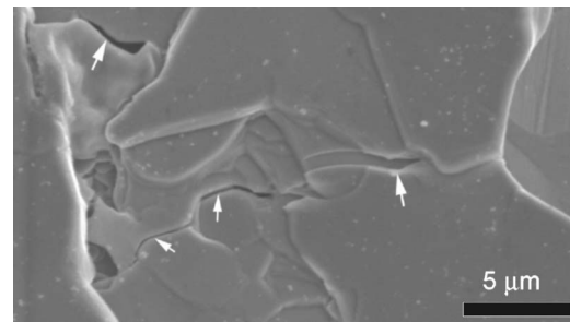
FIG. 2. SEM image of the grain structure of tape B-2 showing crack formation after tensile strain exceeding \epsilon_{\text{irr}} is applied in situ . The arrows indicate some of the cracks. The exact amount of applied strain is unknown due to the partial etching of the tape surface.
