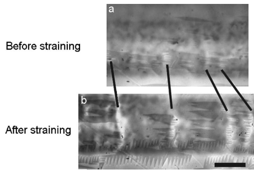
FIG. 1. (a) MO image of part of a filament of tape B-1 before strain is applied. The filament runs horizontally and is partly shielded from the external magnetic field of 25 mT (dark areas). (b) Less dense areas form filament-wide cracks after strain is applied, starting at a strain of \sim 0.61\% . The scale bar is 125 \mu\text{m} long.
