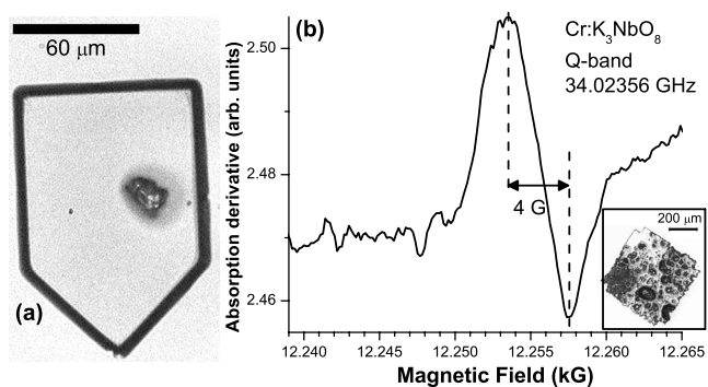
FIG. 3. (a) Photograph of a single crystal of \text{Cr}:\text{K}_3\text{NbO}_8 entrapped in the area delimited by the dark contour. The crystal is encased in optical photoresist, as shown by the gray surface of the contour. (b) Room temperature ESR measurement of diluted \text{Cr}^{5+} spins. The insert shows the actual sample, consisting of few tens of single crystals, in order to achieve a measurable signal by the Q -band spectrometer. The obtained signal is the result of 40 averages, as required by the small size of the signal.
